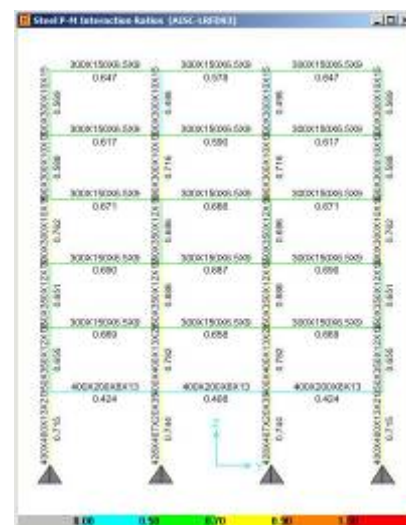
Gambar 13. PM Ratio Portal B - C
