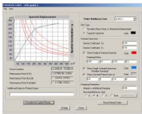
Gambar 19. Arah X, \delta_T = 0.204 m
